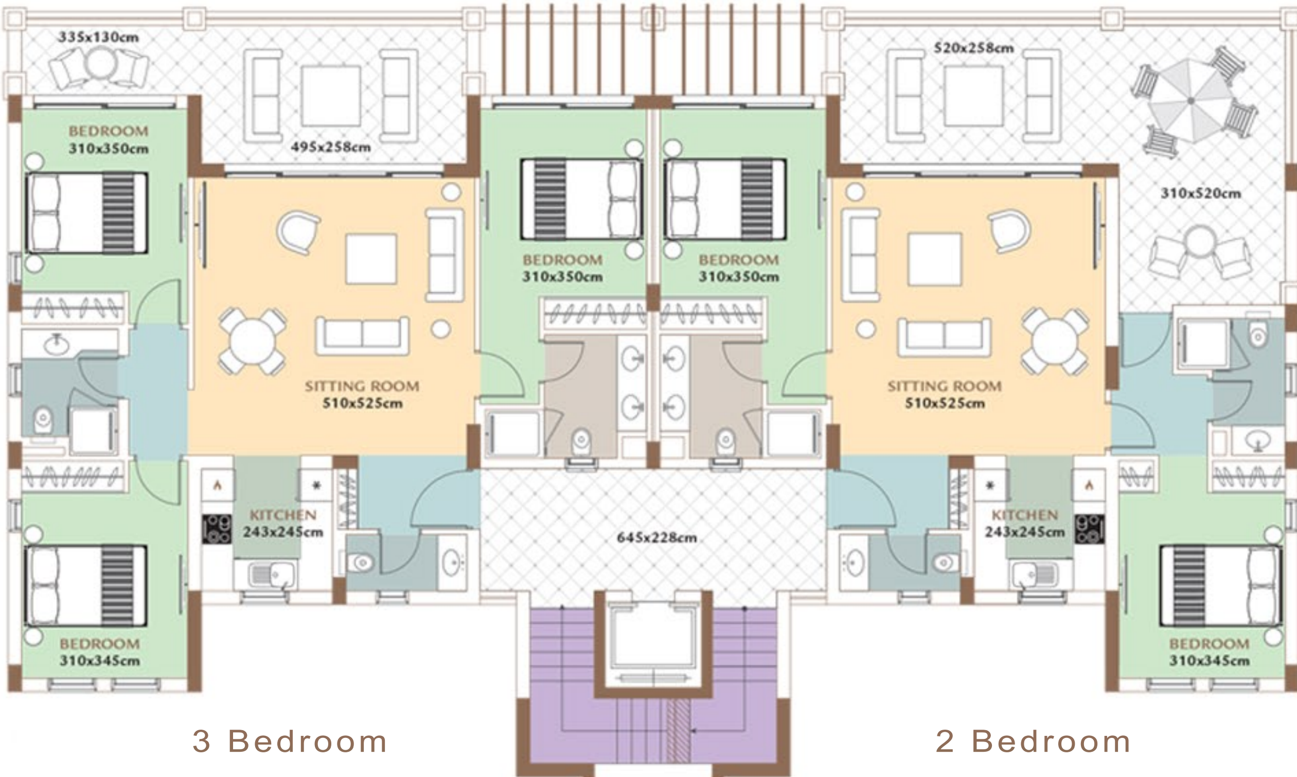
1ST FLOOR
