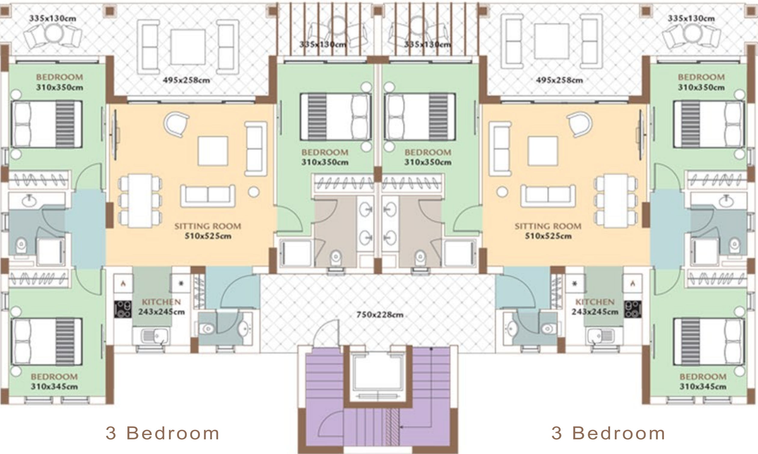
GROUND FLOOR
